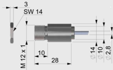
Sensing head
