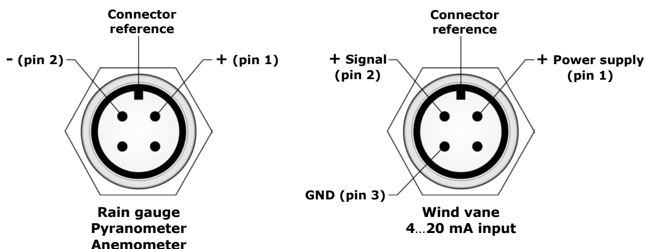
Data logger connectors viewed from outside
