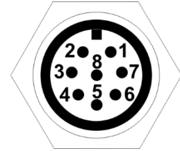
Transmitter male connector
